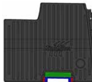
Figure 13 - Passenger Mat Trimming Diagram for kits 105188, 105190, 105192 & 105194
