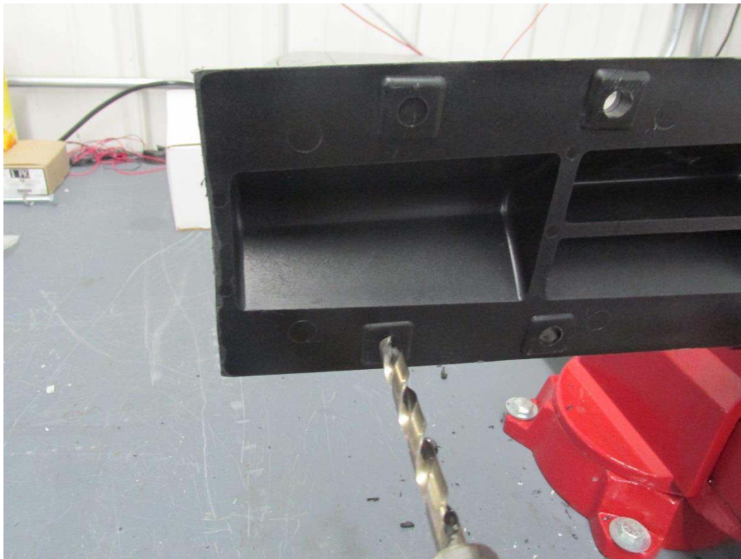
Figure 3 - Drilling Poly Bracket After Trimming
